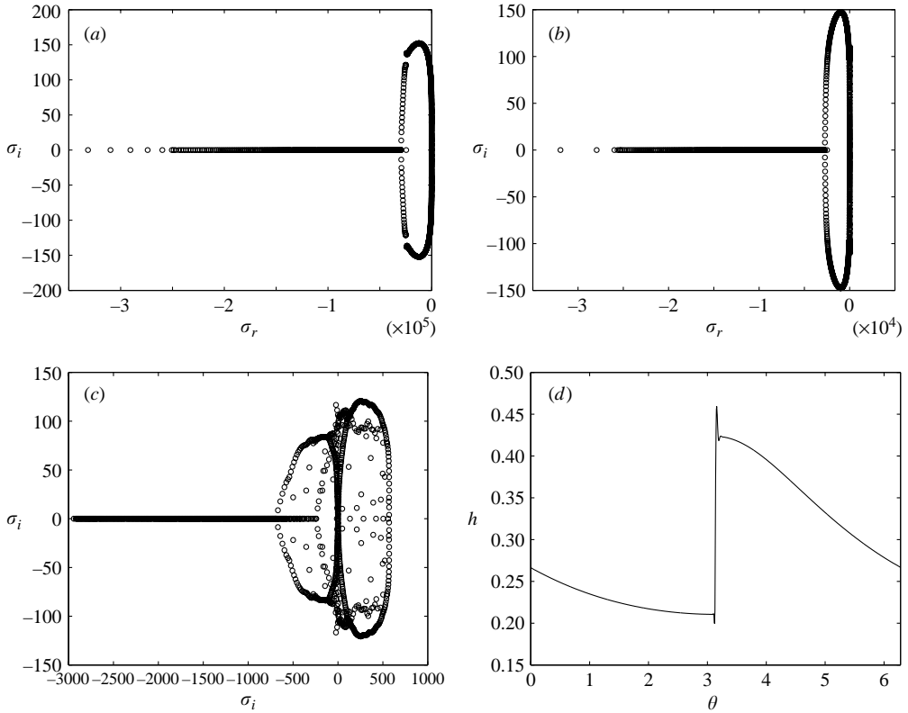
FIGURE 15. Eigenvalue spectrum: q = 0.1359 \approx q_c^0 , \gamma = -3.5 , \delta = 10^{-2} , \bar{h} = 0.29013 , and (a) B^{-1} = 10^{-3} , (b) B^{-1} = 10^{-4} , (c) B^{-1} = 10^{-5} ; (d) the shock profile in case (a).
