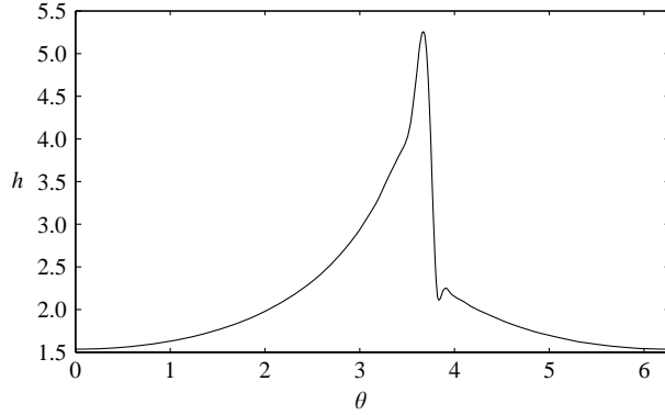
FIGURE 8. A computed single-shock profile at the critical condition: q = q_c^\pi = -3.7976 , \gamma = -3.5 , \delta = 0.0 , B^{-1} = 10^{-5} and \bar{h} = 2.0889 .
